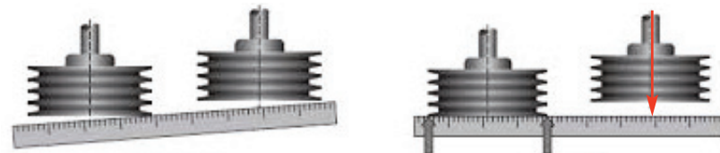
INCORRECT both must be flush on the straight-edge CORRECT
